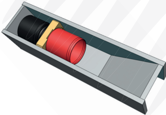
Special reaction arm (in gold (art.nr. 301083)).
